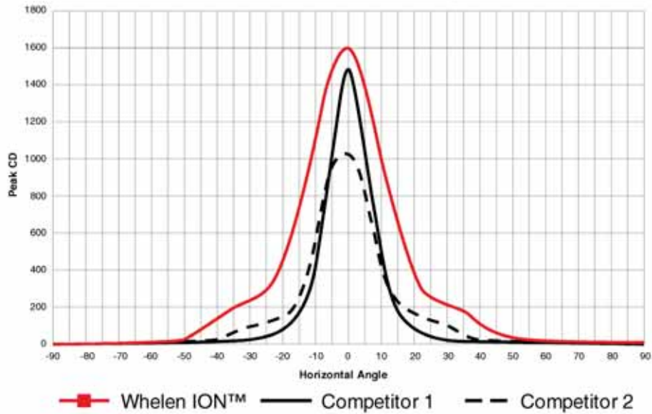
Horizontal angle comparison of the ION against the two leading competitors.
