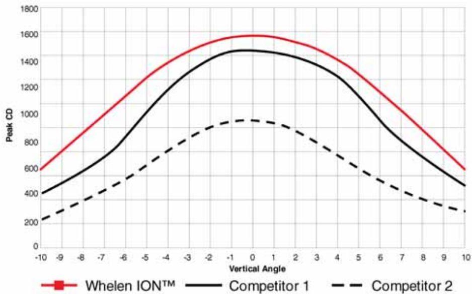
Vertical angle comparison of the ION against the two leading competitors.
